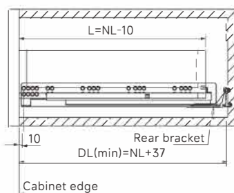
Outset drawer
