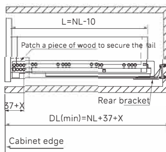
Inset drawer
