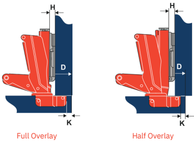
Dimension of hinge cup
