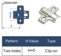
Mounting-plate
