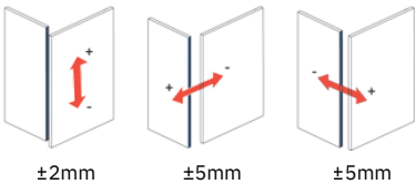
Door adjustment
