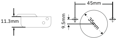
Dimension of hinge cup
