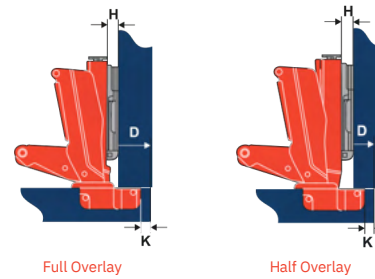
Dimension of hinge cup
