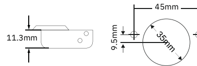
Dimension of hinge cup
