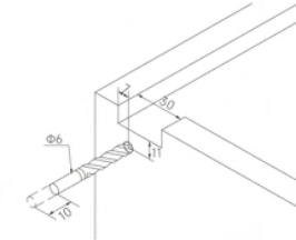
Inset drawer
