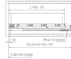
Outset drawer
