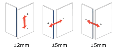
Door adjustment
