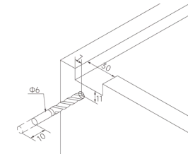
Inset drawer
