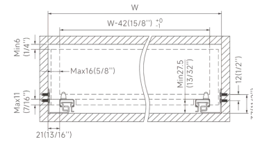
Outset drawer
