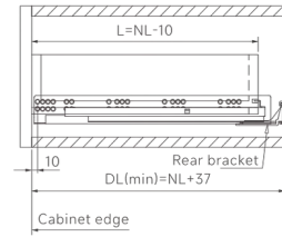
Outset drawer
