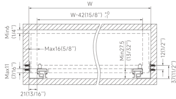
Outset drawer
