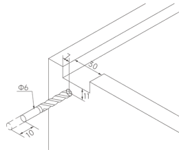
Inset drawer
