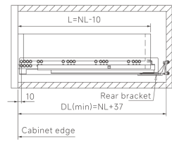
Outset drawer
