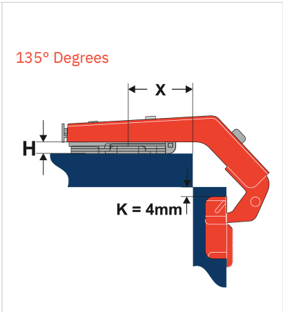
Dimension of hinge cup
