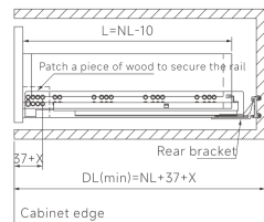
Inset drawer
