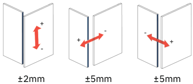
Door adjustment
